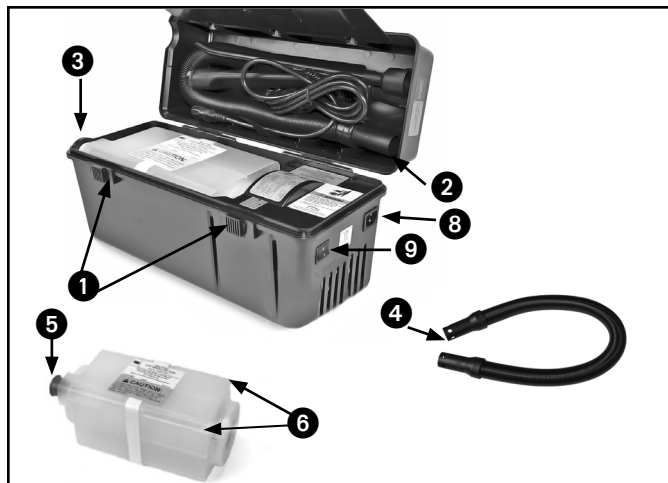
Figure 2. How to operate the 497AJL HEPA Vacuum.
